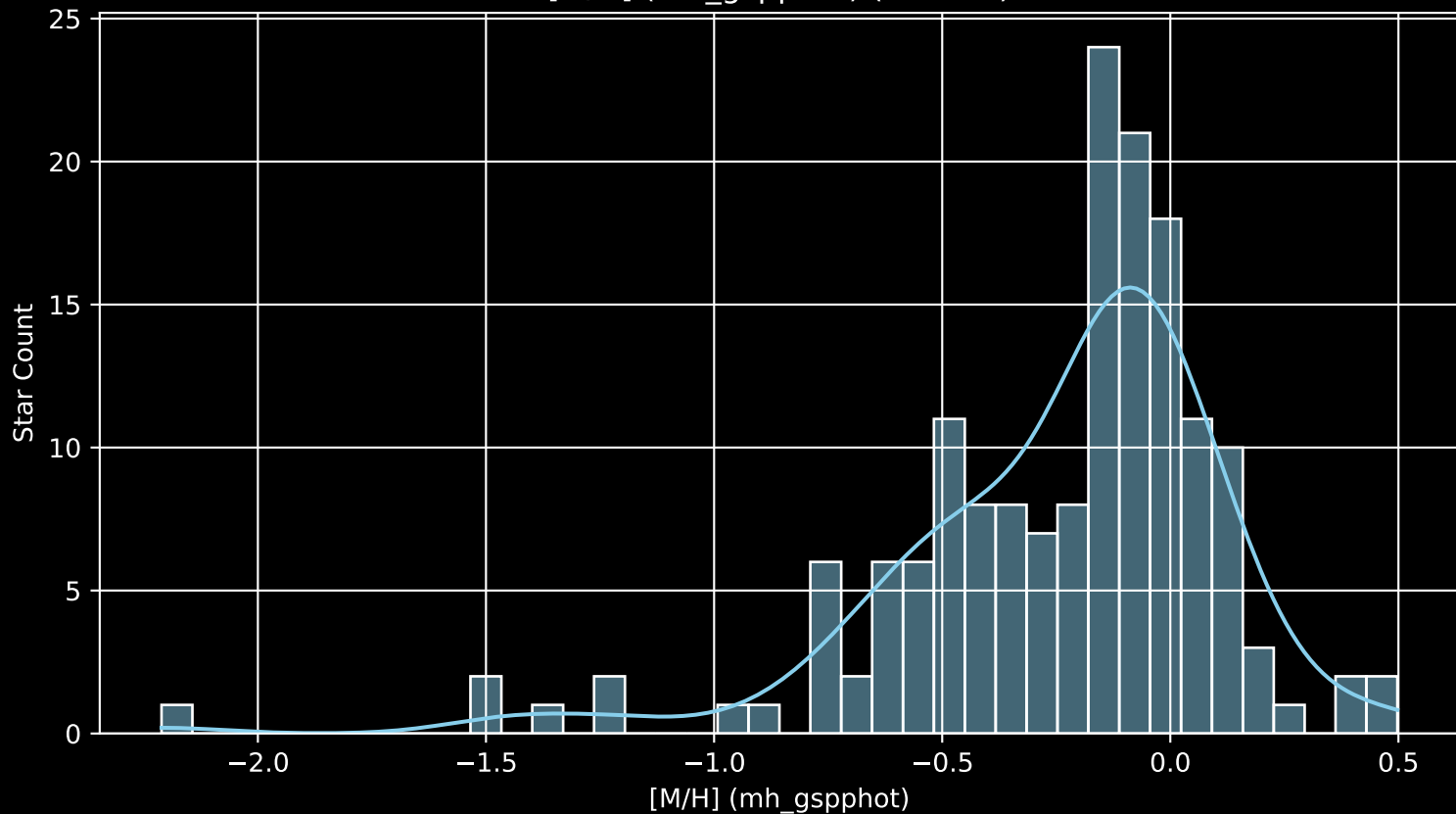
APOGEE DR17 Field: [269-22-O_TESS [M/H] (mh_gspphot) (n= 162)
