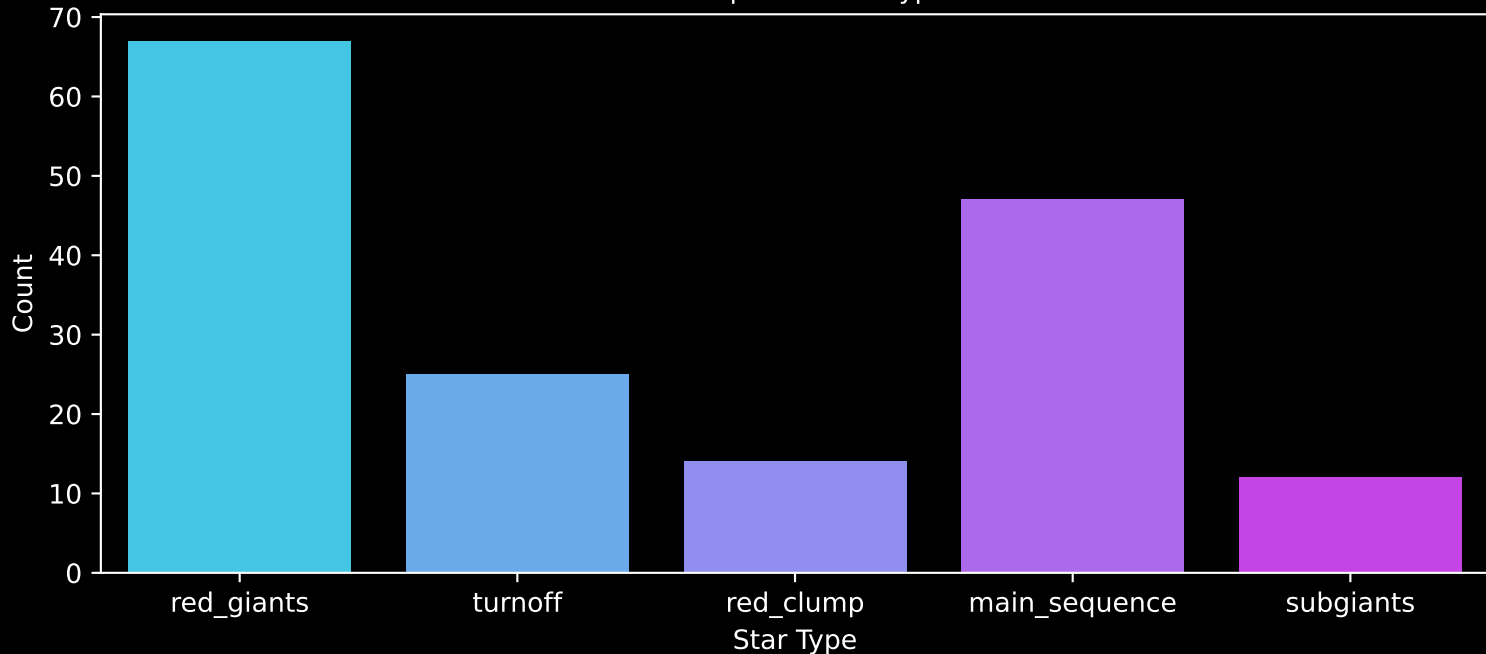
APOGEE DR17 Field: [269-22-O_TESS] Count plot of Star Type
