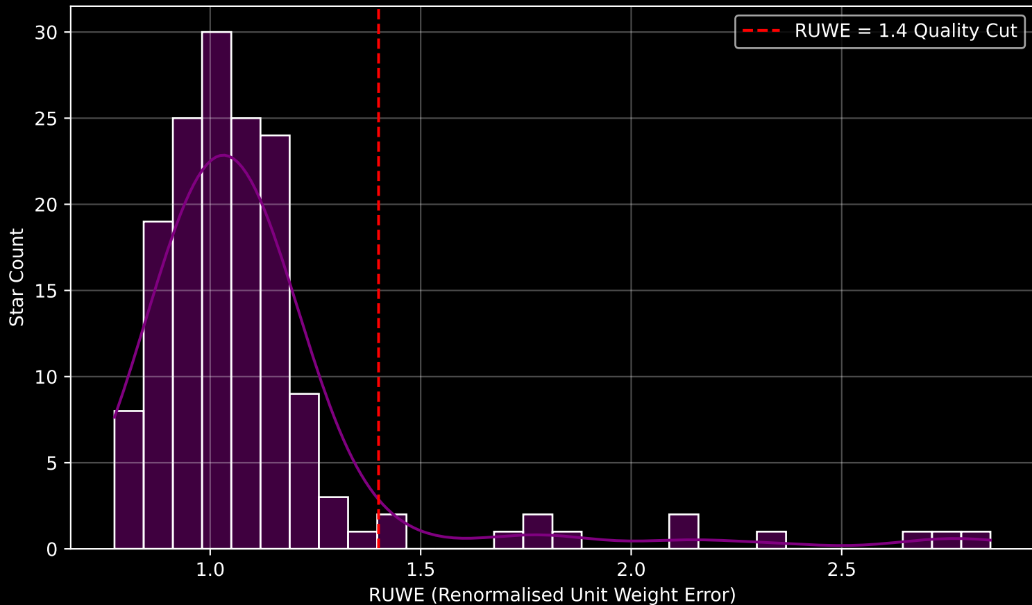
GAPOGEE DR17 Field [269-22-O_TESS] RUWE Distribution (n= 156)
