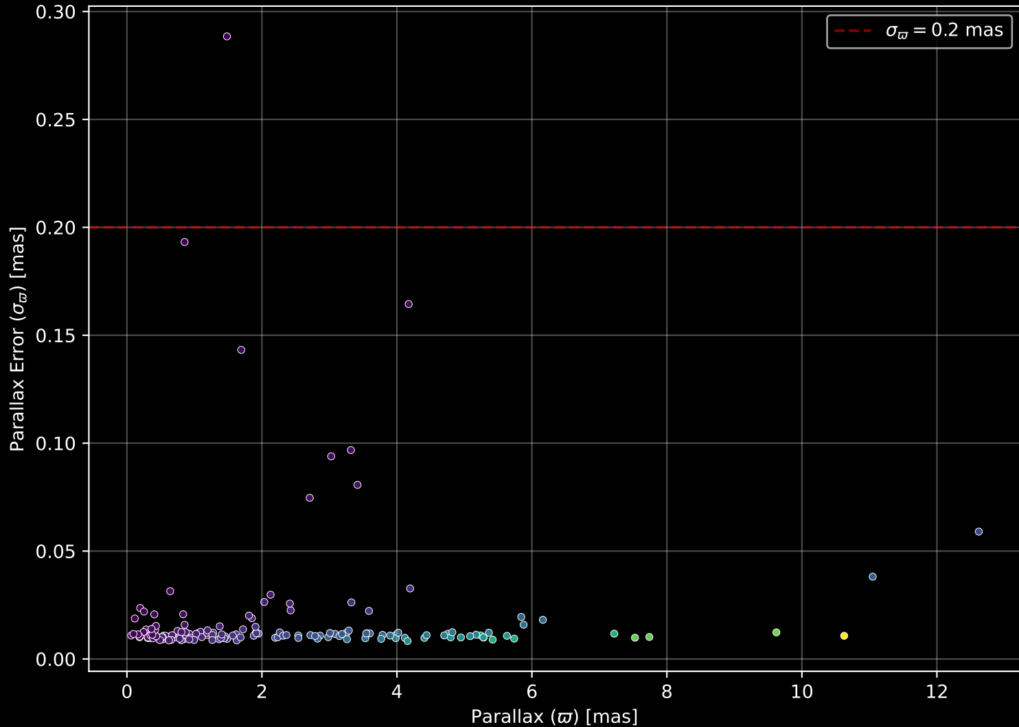
APOGEE DR17 Field: [269-22-O_TESS] Parallax Quality (n= 165)
