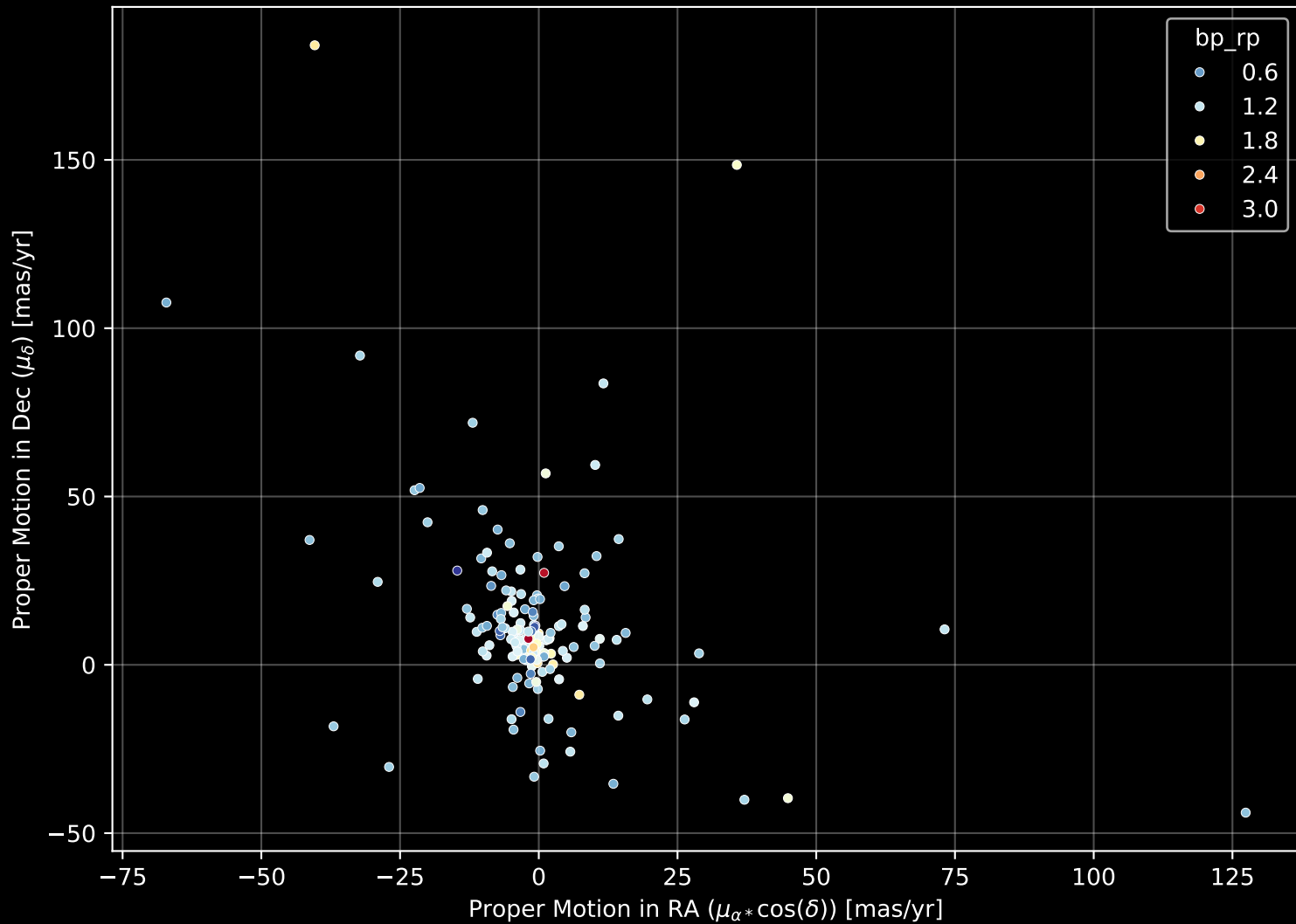
APOGEE DR17 Field: [269-22-O_TESS] Proper Motion Diagram (n= 165)
