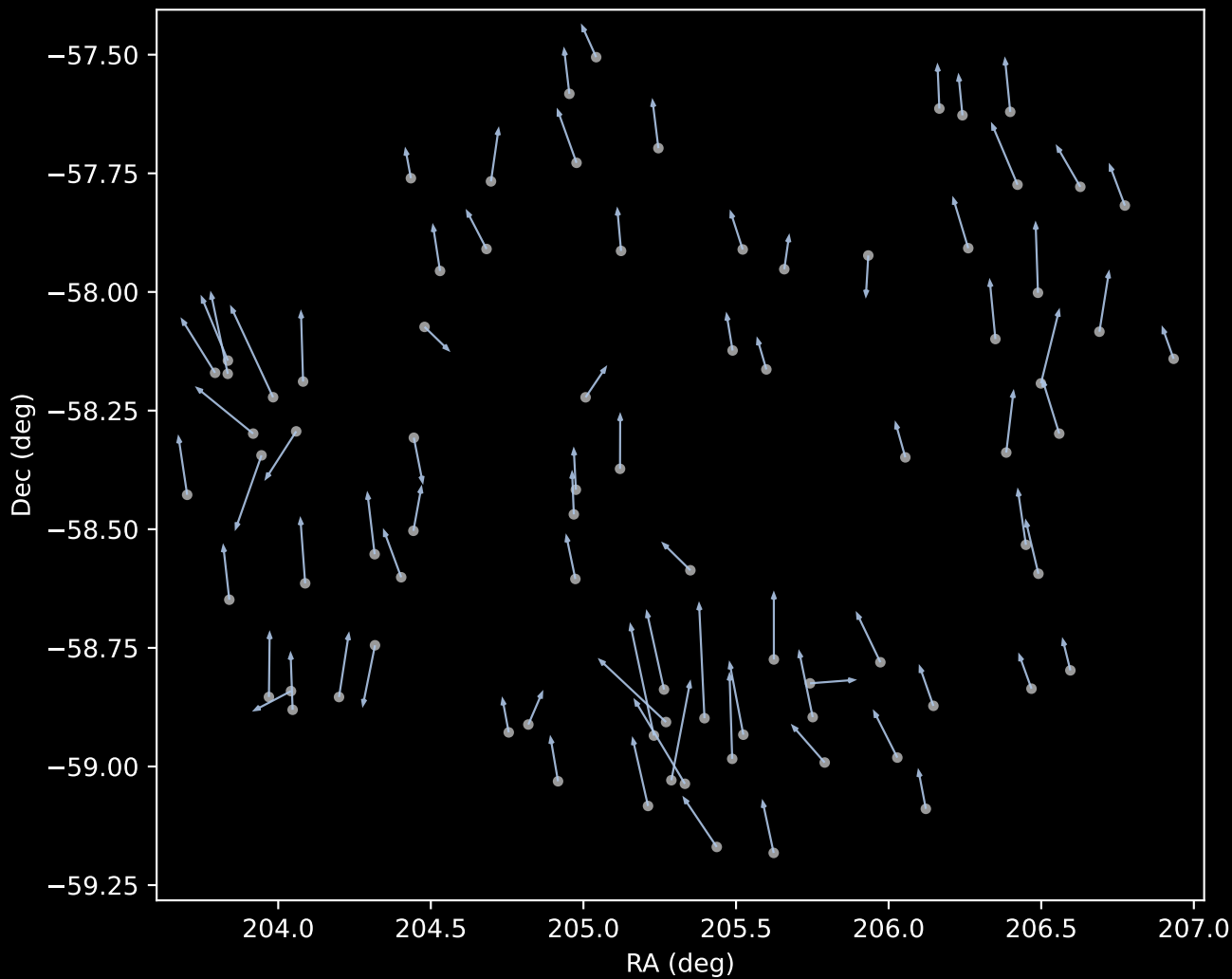
APOGEE DR17 Cluster 1 Proper Motion Vectors (n=82)
